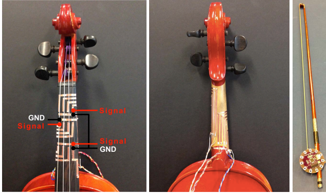
Figure 4. Initial settings for detecting tune of violin play. Each of three positions on the fingerboard has four digital input by four strings, closed the circuits grounded by finger touch.
